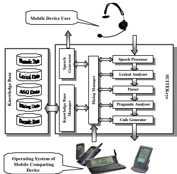
Figure 2. SUITEKeys Architecture
