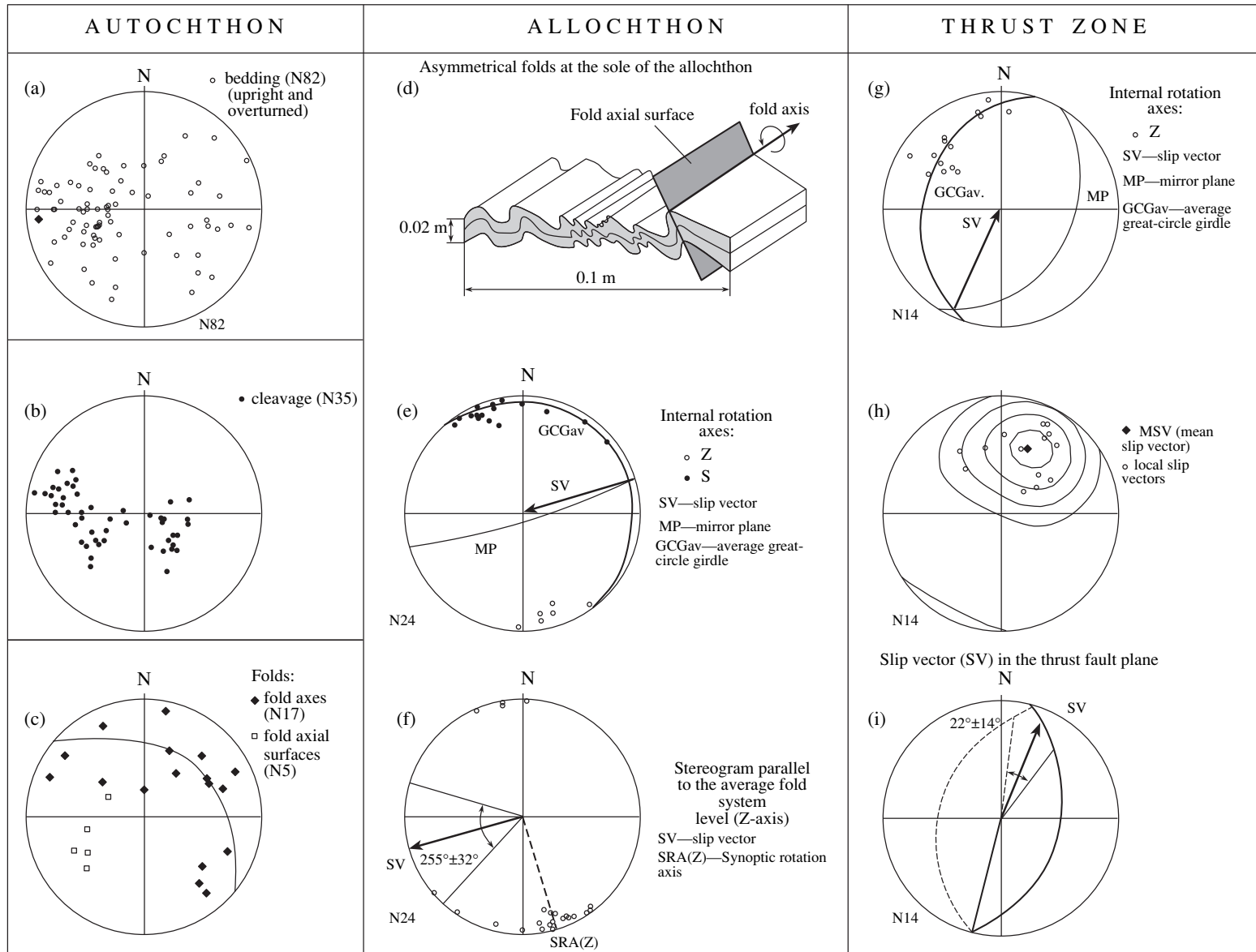
Fig. 11. Structural–kinematic analysis data for the Lesnaya thrust fault (Vatapvayam dome, see Fig. 9). (a)–(c) stereograms: (a) bedding, (b) cleavage, (c) fold axial surfaces and axes; (d) morphology of asymmetrical folds between allochthonous sheets; (e)–(i) stereograms: (e) internal rotation axes for asymmetrical folds; (f) Z-transformed rotation axes for asymmetrical folds projected on the average fold system level; (g)–(i) kinematic analysis in the thrust fault zone (see Fig. 9): (g) internal rotation axes for Riedel structures; (h) dispersion of slip vectors calculated for local Riedel structures; (i) synoptic slip vector on the Lesnaya thrust fault plane in the study area (see Fig. 9). SV—slip vector; the arc shows the confidence angle. Linear and planar features are shown as poles on the Schmidt net, lower hemisphere, except (i). N is the number of structural features of this type used in stereograms.
