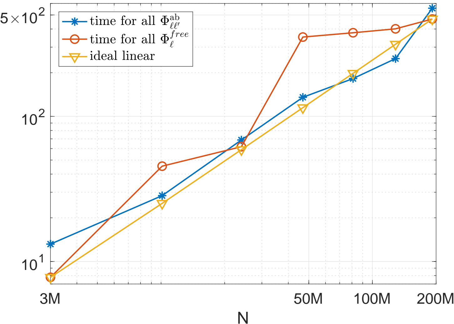
CPU time of FMM for Helmholtz equation in layered media
