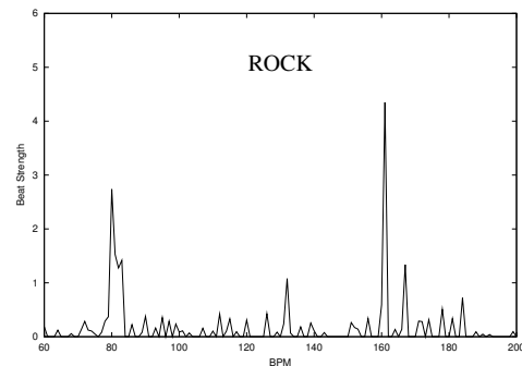
Figure 6: Beat Histogram Example.
