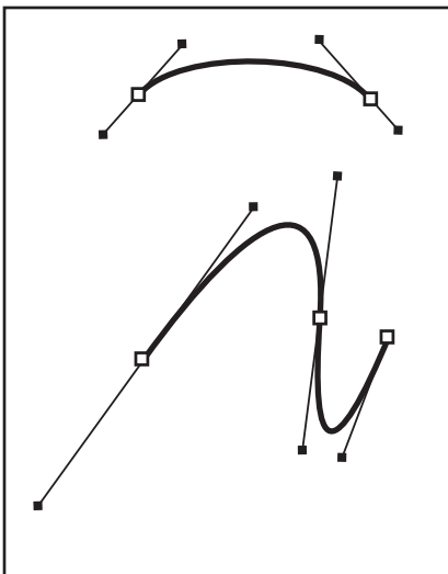
Bézier Handles
