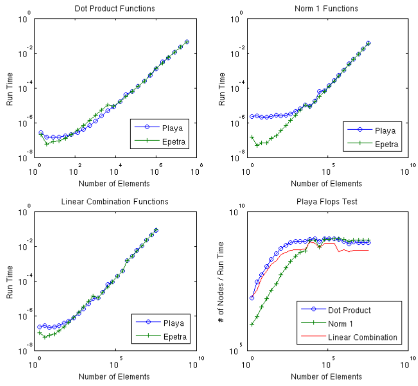
Figure 4: Comparison of Playa and Epetra performance on platform (d)
