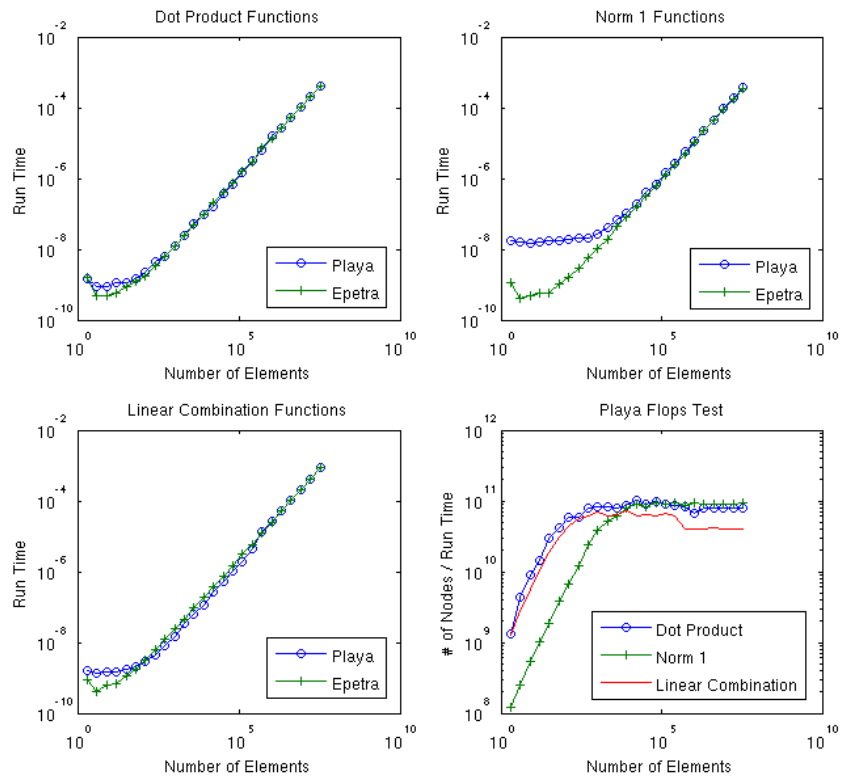
Figure 3: Comparison of Playa and Epetra performance on platform (c)
