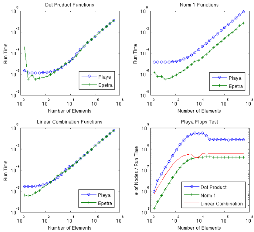
Figure 2: Comparison of Playa and Epetra performance on platform (b)
