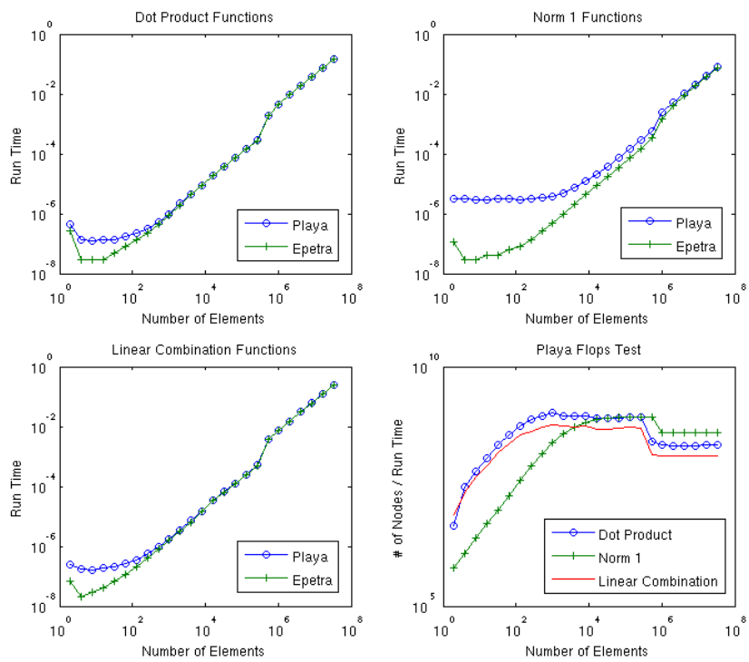
Figure 1: Comparison of Playa and Epetra performance on platform (a)
