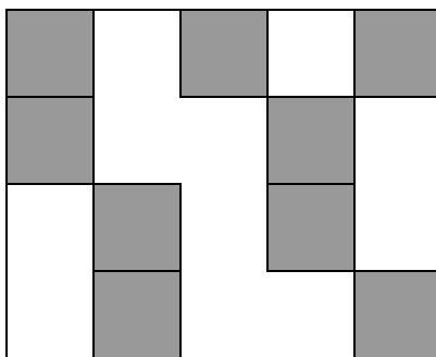
FIGURE 2. Maximally Disjoint Subcollections of Five Intervals
