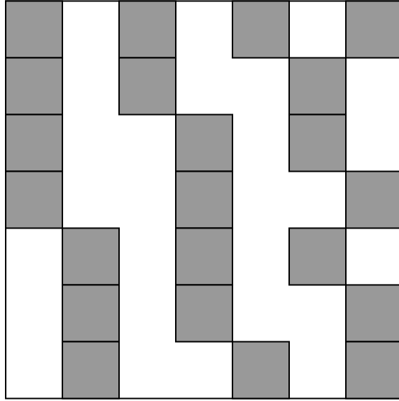
FIGURE 1. Maximally Disjoint Subcollections of Seven Intervals
