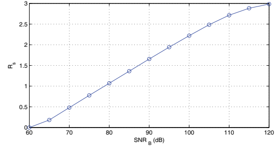
Fig. 6. Achievable secure rate vs. SNR at Bob's receiver while the SNR at Eve's receiver is infinity (Eve has perfect access to the transmitted signal) for r = 10^3 , P = 1 and Bob and Eve applying 10-bit A/D's. Note that the assumption of Eve having a noiseless channel is the extreme case when the eavesdropper has perfect access to the transmitter's output.
