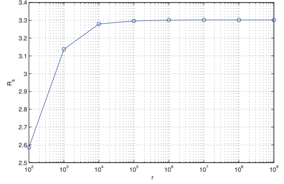
Fig. 3. Achievable secrecy rate versus r (the ratio between the large and the small gain) when both the main and eavesdropper's channels are noiseless and both Bob and Eve apply 10-bit A/D's with the dynamic range a = 2.5 .
