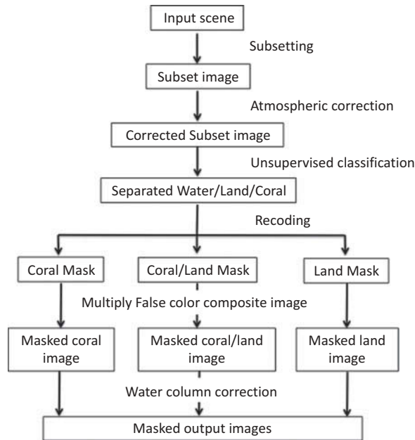
Figure 2. Masking, atmospheric, and water column correction processes for original satellite images for 1987, 2000, and 2013.
