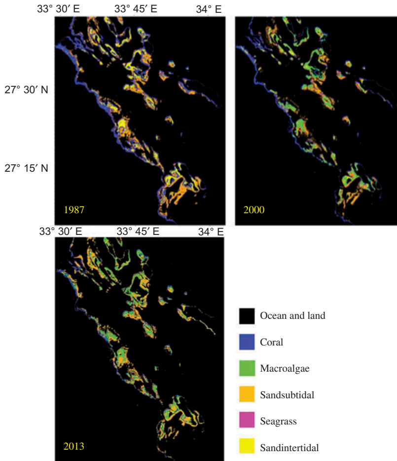
Figure 5. Supervised classification results for coral images from 1987, 2000, and 2013.
