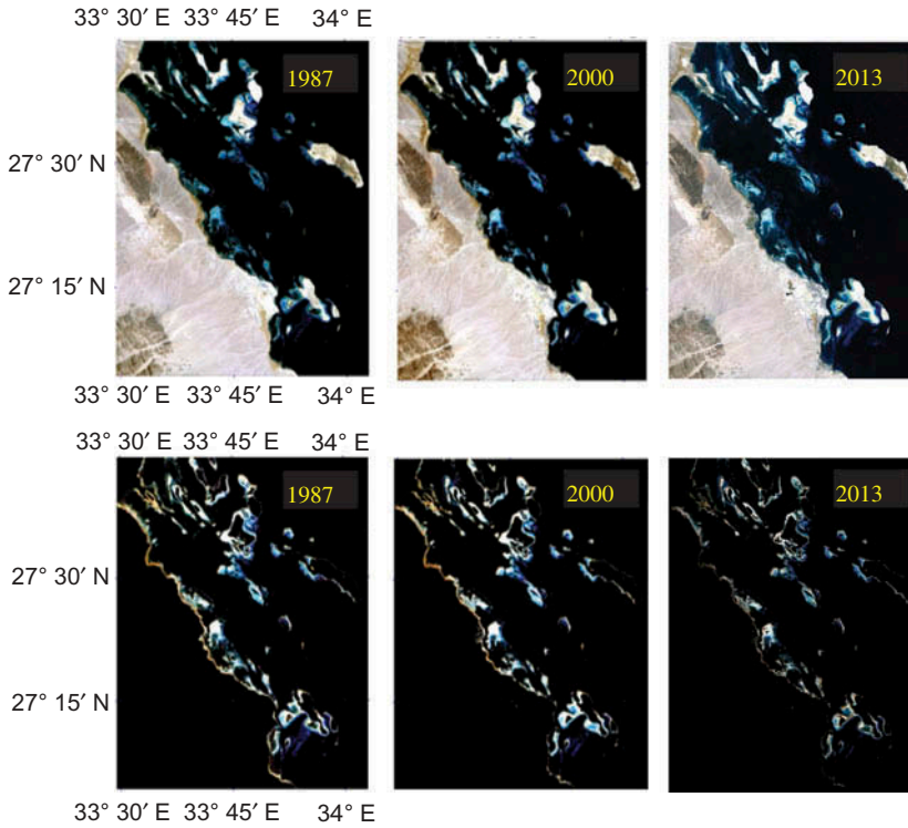
Figure 3. Images from masking process for 1987, 2000, and 2013, Masked coral/land (top), masked coral (bottom) in each pair.
