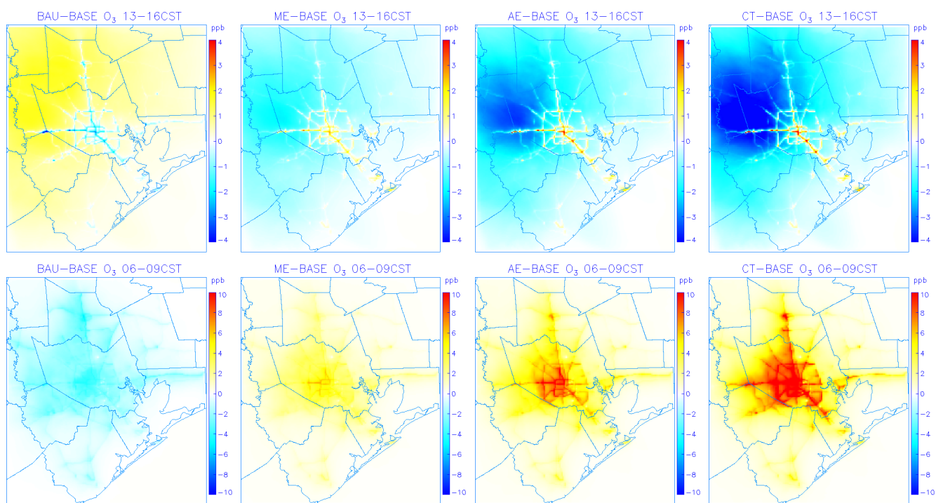
Fig. S8. Simulated O_3 differences during peak time (13-16 CST) and morning rush hour (6-9 CST).
