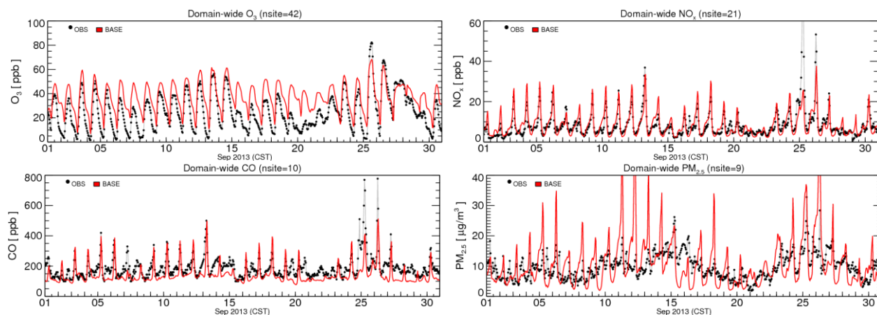
Fig. S3. Time series comparisons of domain-wide surface concentrations of O 3 , NO x , CO, and PM 2.5 between observations (OBS) and Base year simulation (BASE) during September 2013.
