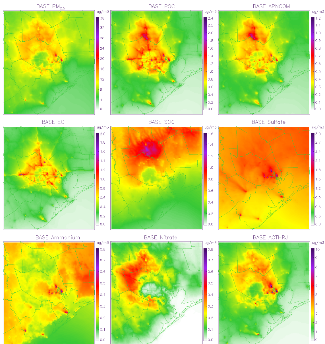
Fig. 7. Spatial distributions of surface concentrations of monthly average \text{PM}_{2.5} and major speciated \text{PM}_{2.5} during September 2013 in the BASE case. (Acronyms: POC - primary organic carbon; APNCOM - primary non-carbon mass; EC - elemental carbon; SOC - secondary organic carbon; AOTHRJ - other unspciated species).
