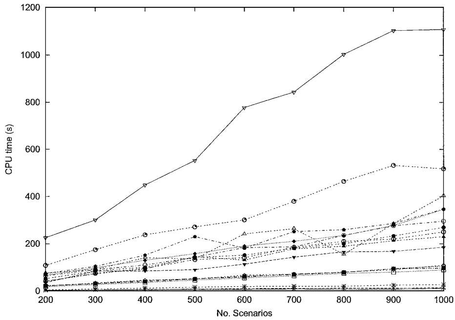
Figure 7. Average CPU times for the SPAF.
