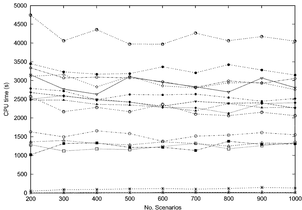
Figure 10. Average CPU times for the TSPRT.
