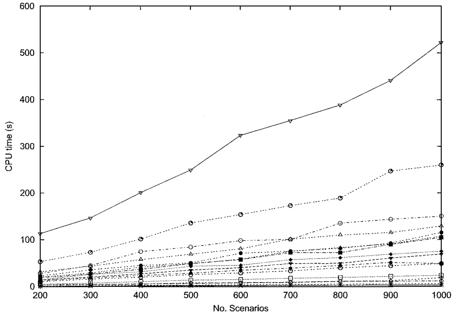
Figure 4. Average CPU times for the SPRT.
