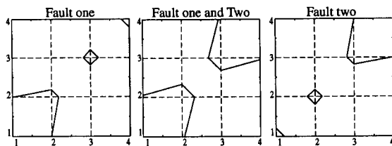
FIGURE 15. The Simulated Correlation Map
