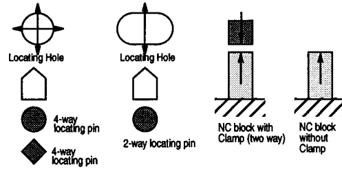
FIGURE 3. Types of locators
