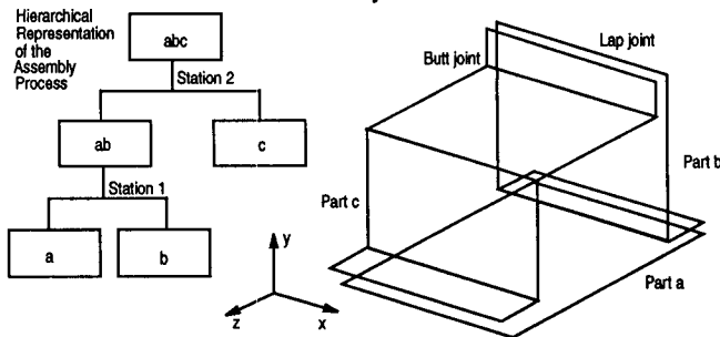
FIGURE 7. Three Parts Assembly
