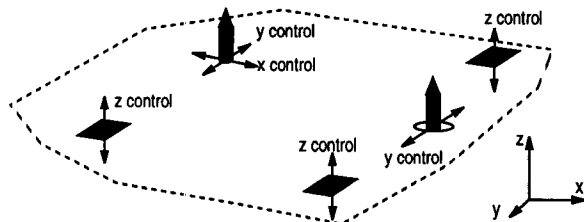
FIGURE 2. A typical 3-2-1 scheme for rigid sheet metal
