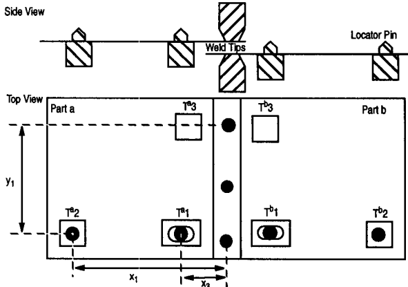
FIGURE 5. Lap-to-Lap joints
