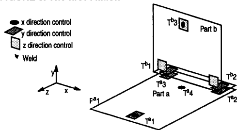
FIGURE 8. The first station
