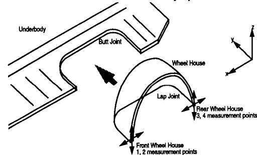
FIGURE 13. Schematic of the assembly operation
