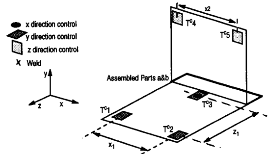
FIGURE 9. The station two and its locating scheme
