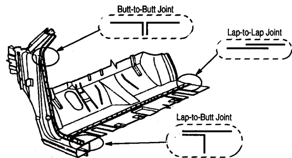
FIGURE 4. Three main types of joints
