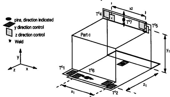
FIGURE 10. Next Station Assembly
