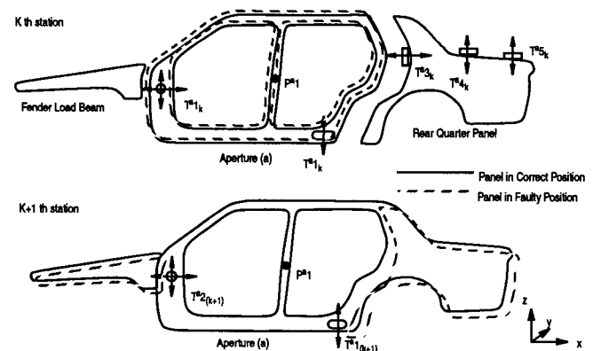
FIGURE 6. An example of the re-orientation concept
