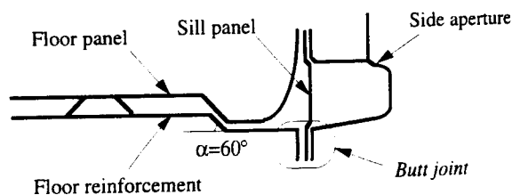
Fig. 4 Design 2: an example of butt joints
