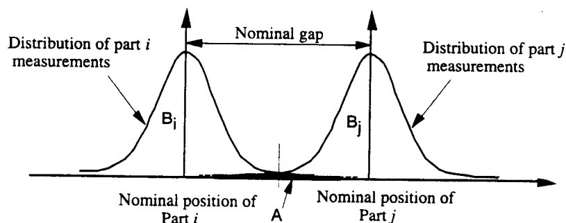
Fig. 6 A model of design gap
