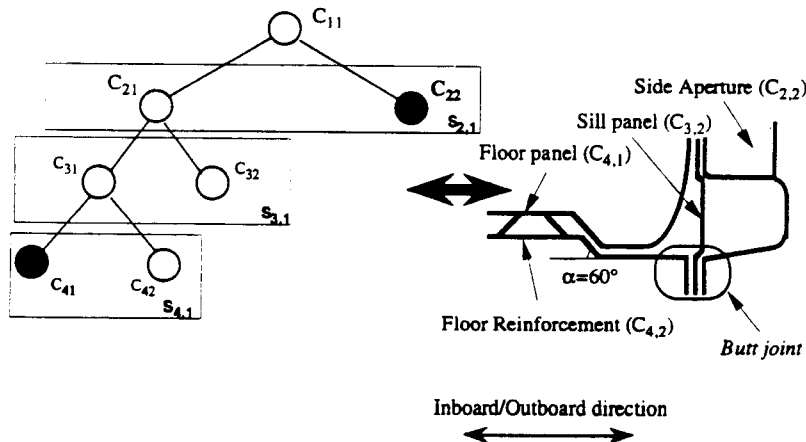
Fig. 11 Design 2: aperture-underbody
