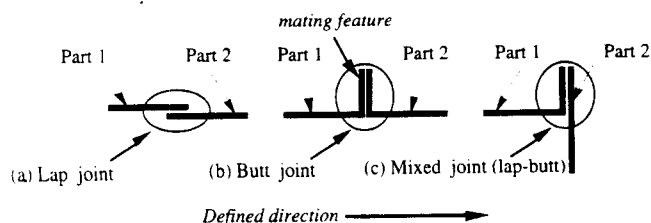
Fig. 2 Cross-sectional views of joint geometries
