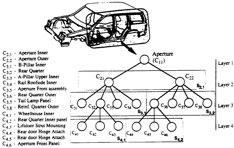
Fig. 7 Example of an automotive body product/process design scheme represented as the hierarchical groups of product/process
