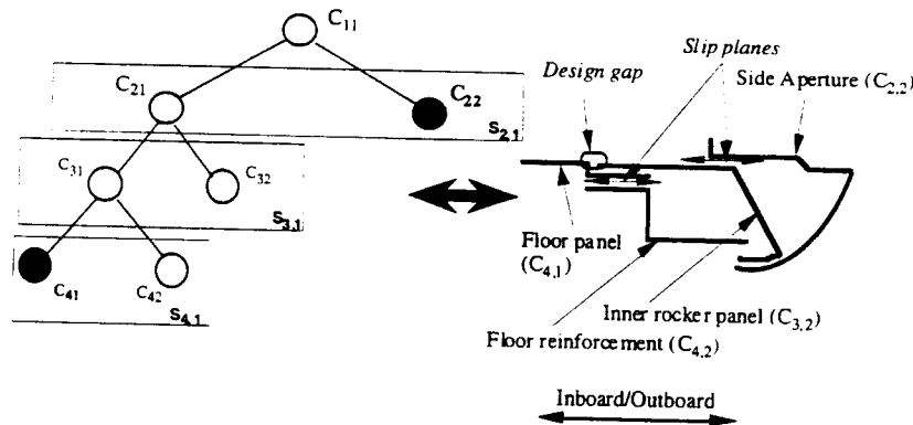
Fig. 10 Design 1: aperture-underbody
