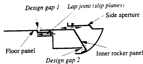
Fig. 3 Design 1: an example of lap joints and a design gap
