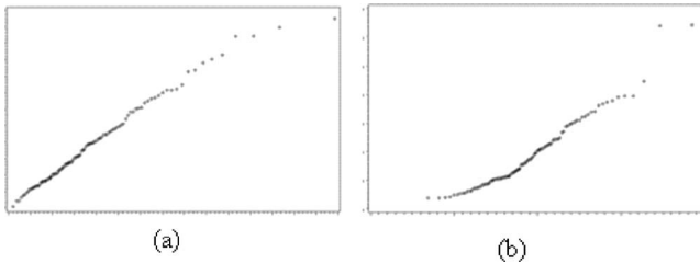
Fig. 8 Chi-square quantile-quantile plot of features (x-axis: chi-square quantiles; y-axis: squared Mahalanobis distances [14] of features; the labels for x- and y-axes are omitted)
