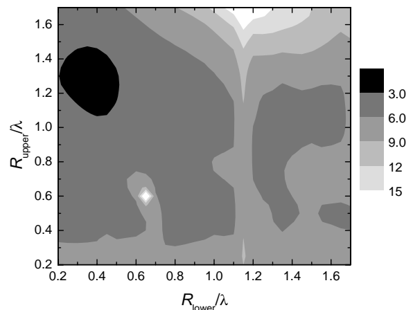
Fig.4. The cost-function in the optimization space.
