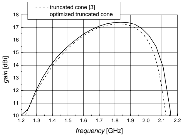
Fig.5. Antenna gain versus frequency.
