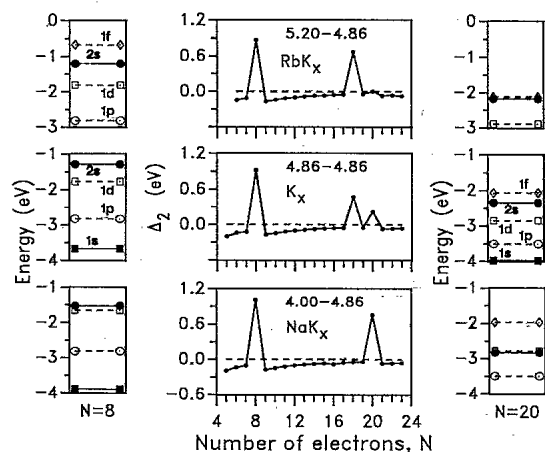
FIG. 5. Jellium second differences for the compound series \text{RbK}_x and \text{NaK}_x ( N = x + 1 ) compared to the pure series \text{K}_x ( N = x ). Bulk Wigner-Seitz radii (as indicated) were used both for the host potassium and for the monovalent impurities. The peak at N = 18 electrons competes with the peak at N = 20 . An impurity with a lower electronic density (higher Wigner-Seitz radius) favors the N = 18 peak and vice versa in accordance with the observations for the mass spectra (Refs. 2 and 33). Notice that the peak at N = 8 is not influenced. This behavior is explained by the relative shift, induced by the impurity, of the 2s level with respect to the other orbitals, as illustrated in the left and right columns. The 2s level is more influenced at N = 20 than at N = 8 . Left column: the jellium single-particle levels at the size N = 8 electrons (solid squares: 1s ; solid circles: 2s ; open circles: 1p ; open squares: 1d ; open diamonds: 1f ). Right column: the jellium single-particle levels at N = 20 electrons.
