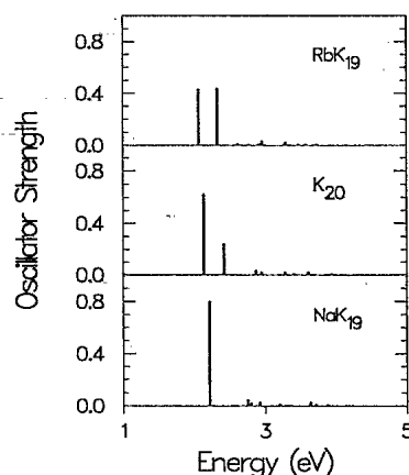
FIG. 9. RPA oscillator strengths for the compound \text{RbK}_{19} , \text{NaK}_{19} , and the pure \text{K}_{20} . Bulk Wigner-Seitz radii were used.
