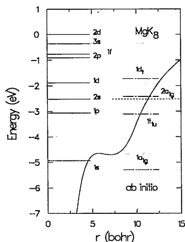
FIG. 4. Comparison of ab initio molecular levels (right) with two-step spherical jellium levels (left) for MgK_8 . The corresponding electronic densities were taken to agree with the bulk values. The agreement between molecular and jellium calculation is very good. Unlike the case of pure K_8 or K_{10} , the 2s level has been shifted below the 1d level and has become the HOMO (dashed line). The jellium effective potential is also shown. Notice the depression that develops at the origin as a result of the Mg impurity.
