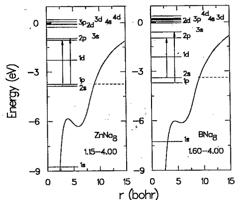
FIG. 13. The variations of the 2s \rightarrow 2p and 1p \rightarrow 3s transitions that develop as the electronic density of the divalent impurity changes. These transitions split the plasmon when the Wigner-Seitz radius of the impurity is 1.15 a.u. (cf. Fig. 12). The associated jellium potentials are also shown. The dashed lines indicate the HOMO levels. The bulk Wigner-Seitz radius of Na that was used is also indicated.
