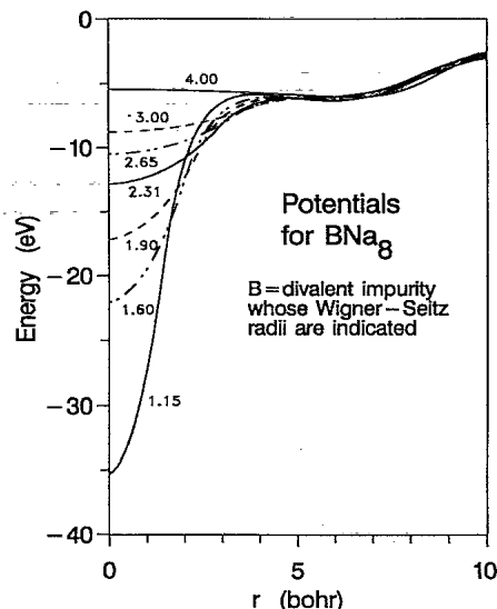
FIG. 11. Jellium potentials for BNa_8 , where B stands for a divalent impurity whose Wigner-Seitz radius varies as indicated from 4.00 to 1.15 a.u.
