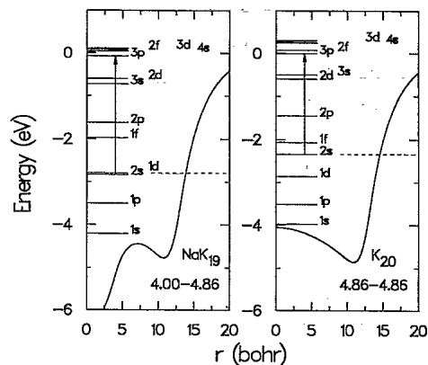
FIG. 8. The variations of the 2s \rightarrow 3p transition that splits the plasmon in the case of pure \text{K}_{20} , but not in the case of the mixed \text{NaK}_{19} . The associated jellium potentials are also shown. The dashed lines indicate the HOMO levels. The bulk Wigner-Seitz radii that were used are also indicated.
