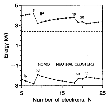
FIG. 1. The ionization potentials (IP's) for the pure series K_x calculated in the spherical jellium approximation. The corresponding energies of the 1p , 1d , 2s , and 1f highest occupied molecular orbitals (HOMO) are also shown. The maximum IP's appear when an electronic shell is closed at N = 8 , 18, and 20 electrons ( N = x ). All the IP's have values higher than the bulk work function of potassium at 2.4 eV (dashed line).
