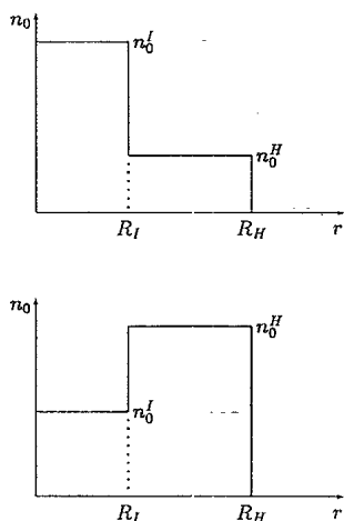
FIG. 3. Schematic representation of the two-step positive jellium background, with the impurity ( I ) occupying the central region. Both cases of an impurity with a larger ( n_0^I > n_0^H ) and a smaller ( n_0^I < n_0^H ) electronic density than the host are shown.
