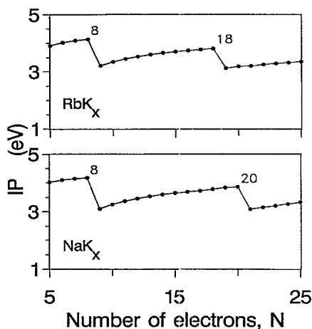
FIG. 7. The ionization potentials for the compound series \text{RbK}_x and \text{NaK}_x ( N = x + 1 ). Compared to the pure \text{K}_x (cf. Fig. 1), only one step appears in the range N = 18 – 20 . N = 18 is favored over N = 20 for \text{RbK}_x , while the opposite holds for \text{NaK}_x .
