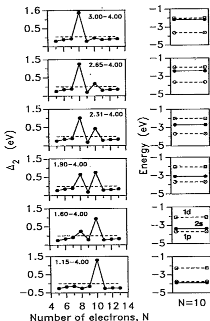
FIG. 10. Left column: jellium second differences for the series BNa_x ( N = x + 2 ), where B denotes a divalent impurity whose Wigner-Seitz radius varies from 3.00 to 1.15 a.u., as indicated in the figure. Right column: jellium single-particle spectra for BNa_8 corresponding to the different electronic densities of the divalent impurity (solid circles: 2s ; open circles: 1p ; open squares: 1d ). The downward shift of the 2s orbital between the 1d and the 1p levels is apparent, and correlates with the variations in the second differences. The r_s that best reproduce the observations (cf. Table III) for the mass spectra of ZnNa_x are 1.15 and 4.00.
