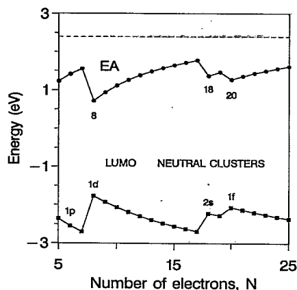
FIG. 2. The electron affinities (EA's) for the pure series K_x calculated in the spherical jellium approximation. The corresponding energies of the 1p , 1d , 2s , and 1f lowest unoccupied molecular orbitals (LUMO) are also shown. The minimum EA's appear when an electronic shell is closed at N = 8, 18, \text{ and } 20 electrons ( N = x ). All the EA's have values lower than the bulk work function of potassium at 2.4 eV (dashed line).
