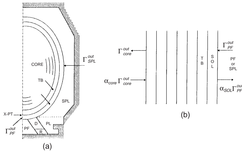
Figure 1. Schematic diagram of the neutral transport model: (a) 2-D TEP model of divertor plasma (D), recycling region (R), private flux (PF), plenum (PL) and SOL plenum (SPL); (b) 1-D ICB model of penetration through SOL and transport barrier (TB) into core.
