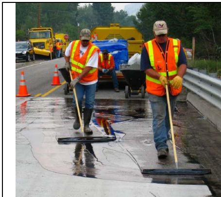
Deck Sealing
