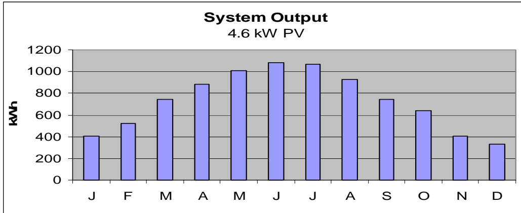
Figure 8: PV System Output
