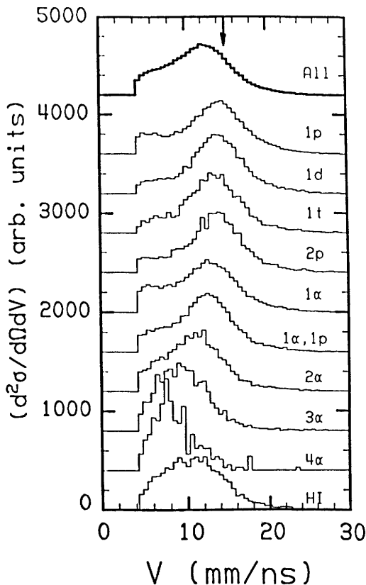
Figure 1. The channel decomposition of the velocity distribution of fusion-like products. The channels are labeled by the type and number of the forward particles. The top (bold) distribution is the sum of all charged particle channels. The distributions are offset from the abscissa for display. The arrow indicates V_{full} .
