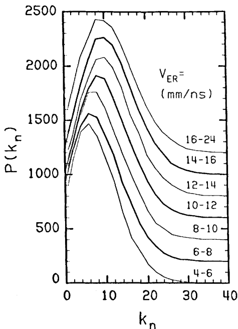
Figure 5. Neutron fold distributions for seven residue velocity bins. These distributions are deduced from the backward, \theta_{lab} > 75^\circ , NaI detectors with an overall solid angle correction to account for the solid angle with \theta_{lab} < 75^\circ . The distributions are offset from the abscissa for display.
