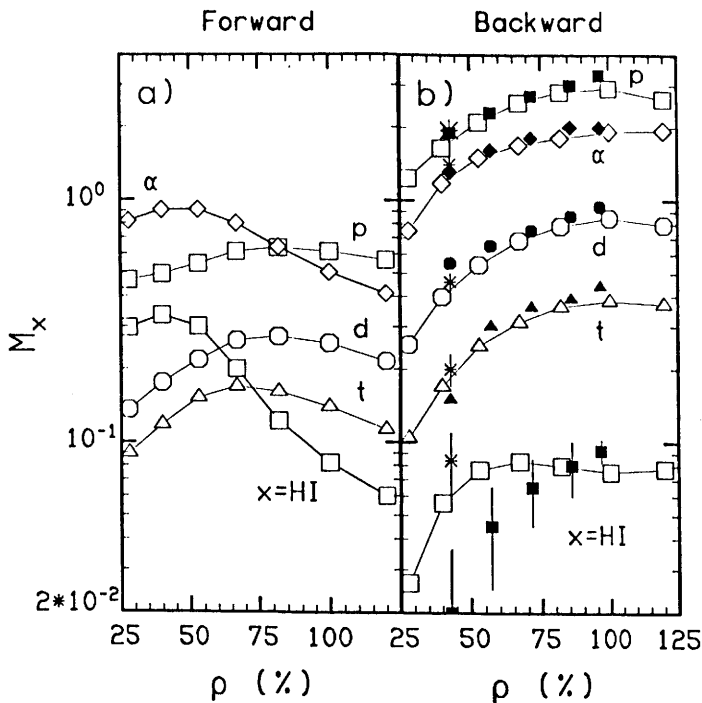
Figure 4. The multiplicities of charged particles detected at a) forward ( \theta < 35^\circ ) and b) backward ( \theta > 35^\circ ) angles as a function of the linear momentum transfer. The open symbols are derived from inclusive charged particle-residue coincidences. The solid and star symbols are derived from a subset of the inclusive data where specific exclusive channels (forward particles) are selected, see text.
