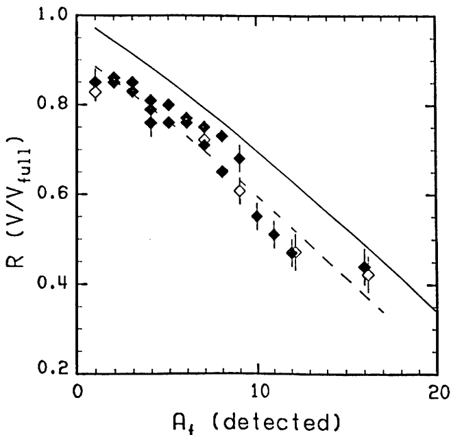
Figure 2. Ratio of velocity centroid of the channel selected data to the value for complete momentum transfer. The abscissa ( A_f ) corresponds to all detected forward mass (solid diamonds) and to the detected forward mass with energies greater than the evaporation peak (open diamonds). The solid line is the result of a calculation assuming a linear momentum deficit equal to A_f \times the beam momentum per nucleon. The dashed curve assumes 3 additional beam velocity nucleons (neutrons) exist in each channel but are not observed.
