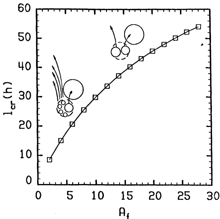
Figure 6. The critical angular momentum values for the ^{28}\text{Si} + ^{100}\text{Mo} system as a function of exit channel mass asymmetry. In this calculation the remainder of the projectile fuses. The values of l_{cr} are almost identical if the remainder of the projectile is neglected, presumed not to fuse.
