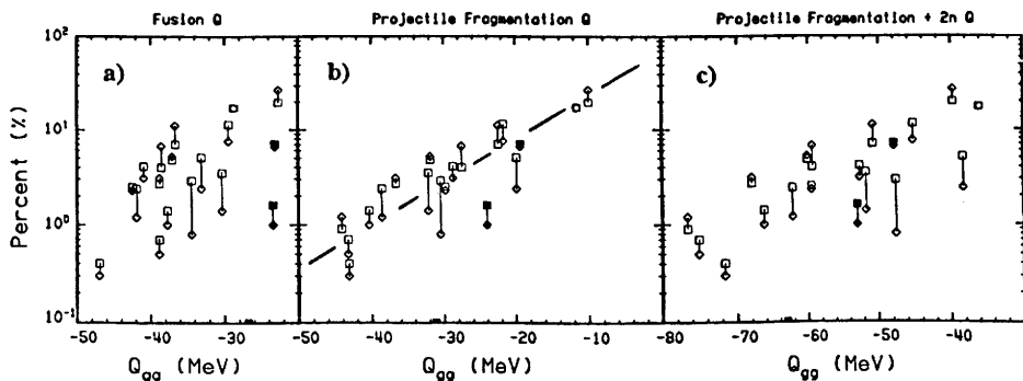
Figure 3. Correlation between channel probability and Q-value. Channels defined by all forward particles regardless of kinetic energy are represented by squares. Channels defined only by particles with energies in excess of the evaporation peak are represented by diamonds. The solid symbols are for the 2\alpha , 3\alpha , and 4\alpha channels. Table I contains a list of the channels. The abscissa for a) is the Q-value for incomplete fusion (eq. 1), b) is the Q-value for projectile fragmentation (eq. 2), and c) is the Q-value for projectile fragmentation with 2 additional free neutrons.
