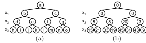
Figure 2: Search Tree
