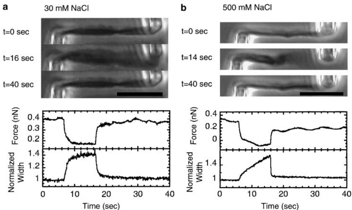
Fig. 2. Images of combined chemical–micromechanical experiments with 30 mM NaCl (a), 500 mM NaCl (b), 20 mM \text{MgCl}_2 (c), 300 mM \text{MgCl}_2 (d), and 40 mM \text{Co}(\text{NH}_3)_6\text{Cl}_3 (e). The images show the chromosome before, during, and after an exposure to the different ionic conditions. The plots show the time series of the force the chromosome supports and width of the chromosome. For 30 and 500 mM NaCl, the force decreases and the width increases. However, 20 mM \text{MgCl}_2 induces an increase in the force and decrease in width. 300 mM \text{MgCl}_2
