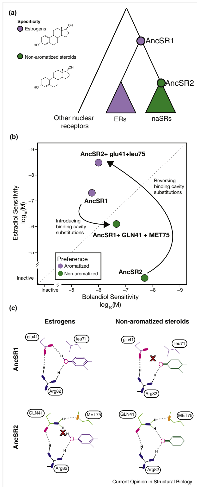
Evolution of ligand specificity in vertebrate steroid receptors [40,45]. (a) Evolutionary relationship of estrogen receptors (ERs) and non-aromatized steroid receptors (naSRs). Circles represent reconstructed
