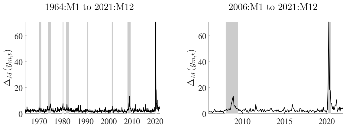
Figure 1: Extreme Monthly Observations: Mahalanobis Distance
