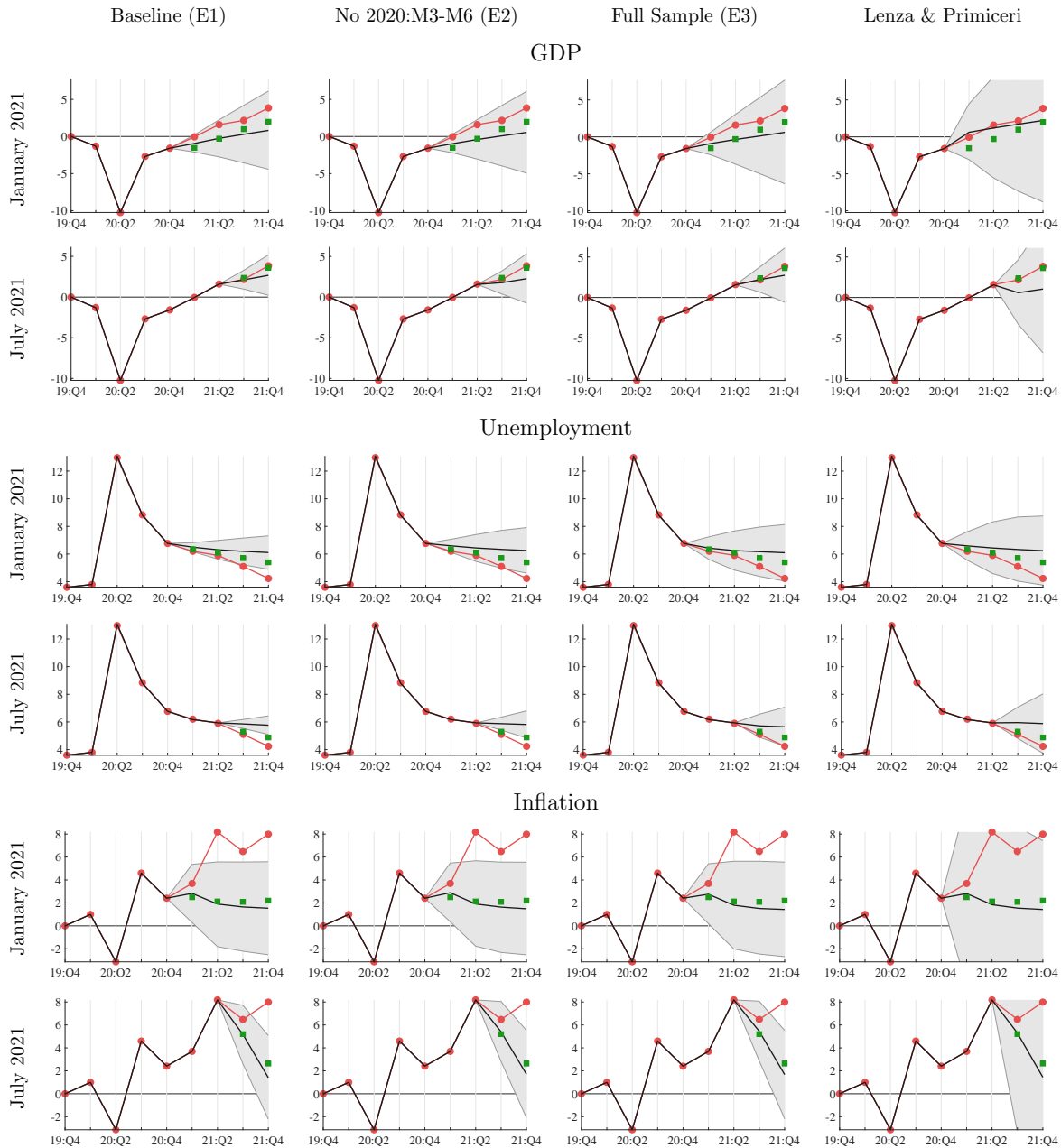
Figure 8: January and July Forecasts for 2021
