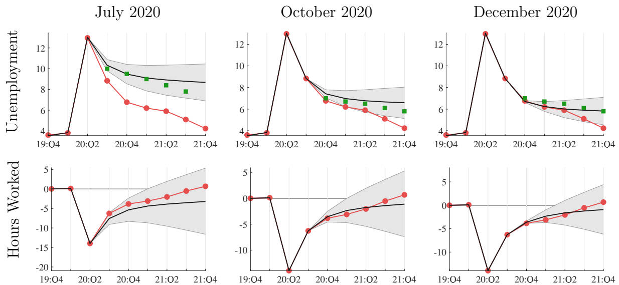
Figure 6: Labor Market Forecasts in 2020:Q3 and Q4
