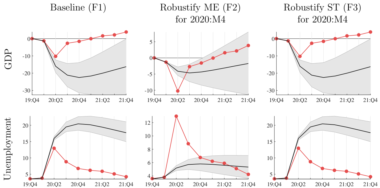
Figure 4: Effect of Filtering on Forecasts in May 2020
