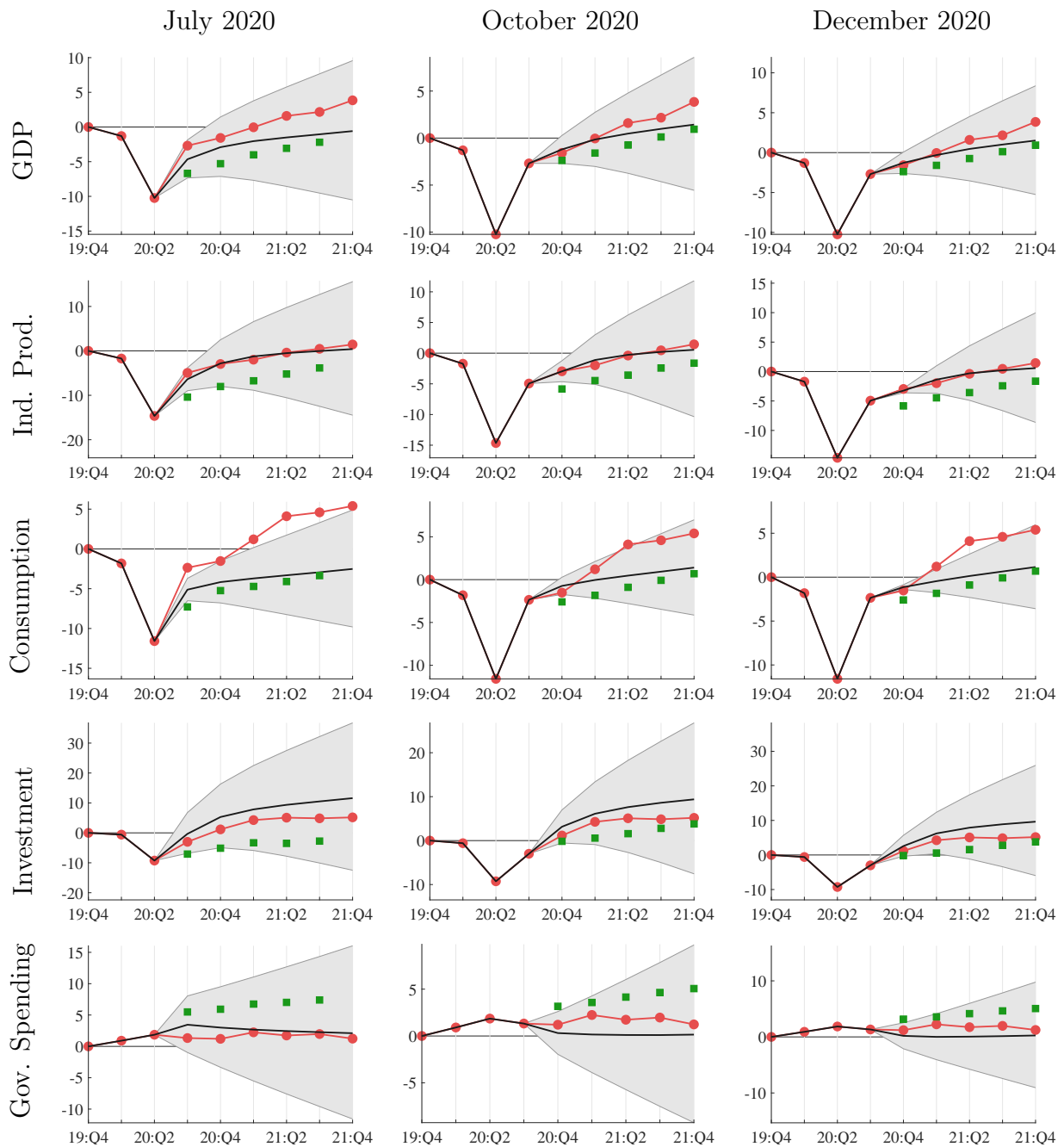
Figure 5: Real Activity Forecasts in 2020:Q3 and Q4
